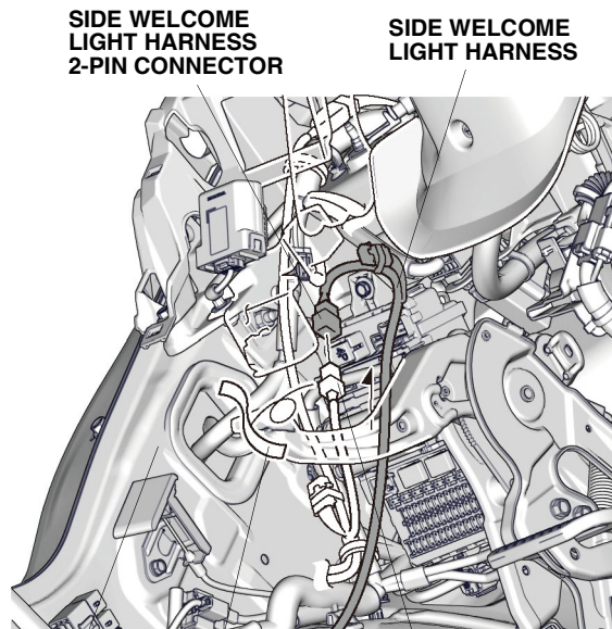
DRIVER'S KICK PANEL OPENING
