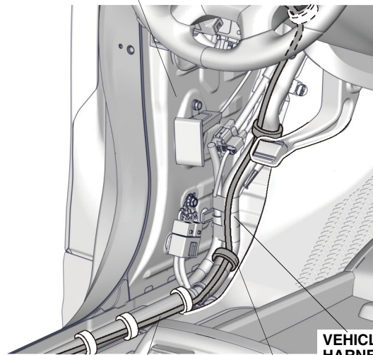
SIDE WELCOME LIGHT HARNESS
