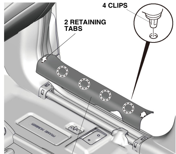
PASSENGER'S DOOR SILL TRIM
