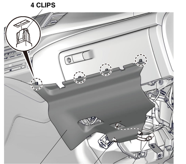
PASSENGER'S DASHBOARD UNDER COVER 2 PINS VEHICLE CONNECTOR (if equipped)
