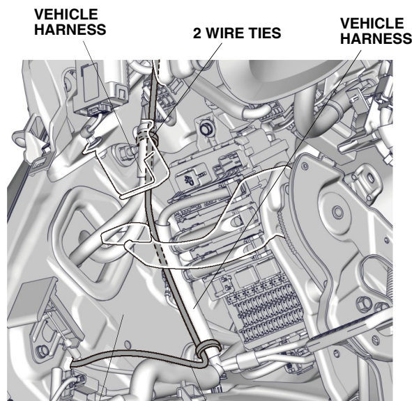
DRIVER'S KICK PANEL OPENING
