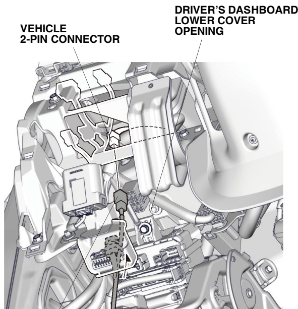
SIDE WELCOME LIGHT HARNESS 2-PIN CONNECTOR
